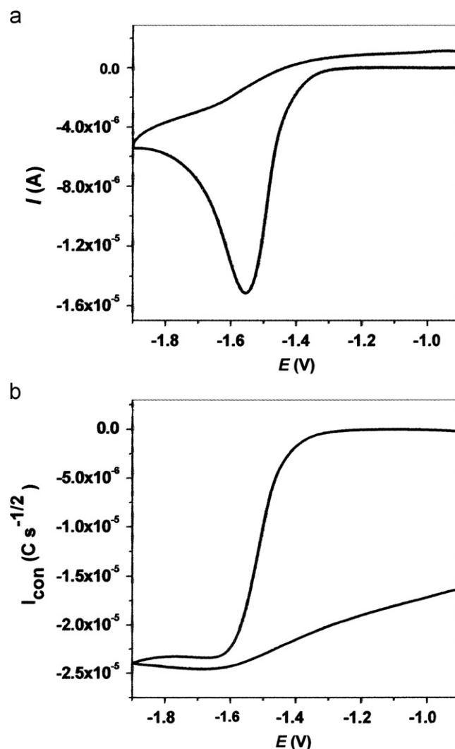
Fig. 1. Cyclic (a) and convoluted cyclic (b) voltammograms of PAT in ACN+0.1 mol L -1 TBAP. c_{\text{PAT}}^*=5.2 \times 10^{-4}\text{ mol L}^{-1} , v=0.075\text{ V s}^{-1} .
