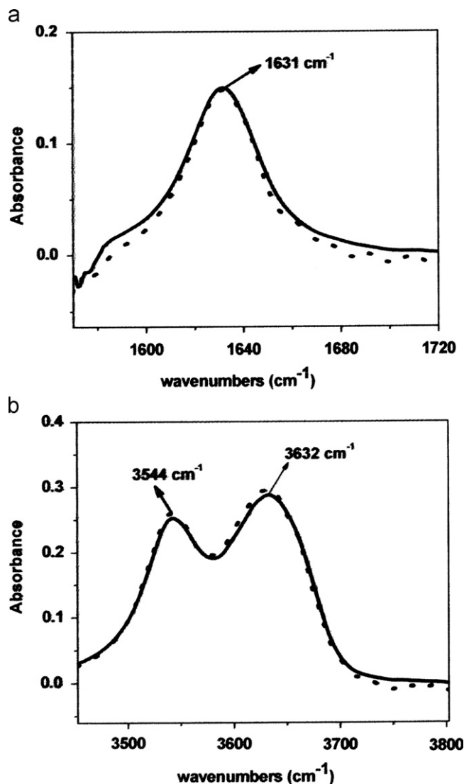
Fig. 3. IR spectra recorded before (solid line) and after (dotted line) performing the controlled potential electrolysis.
