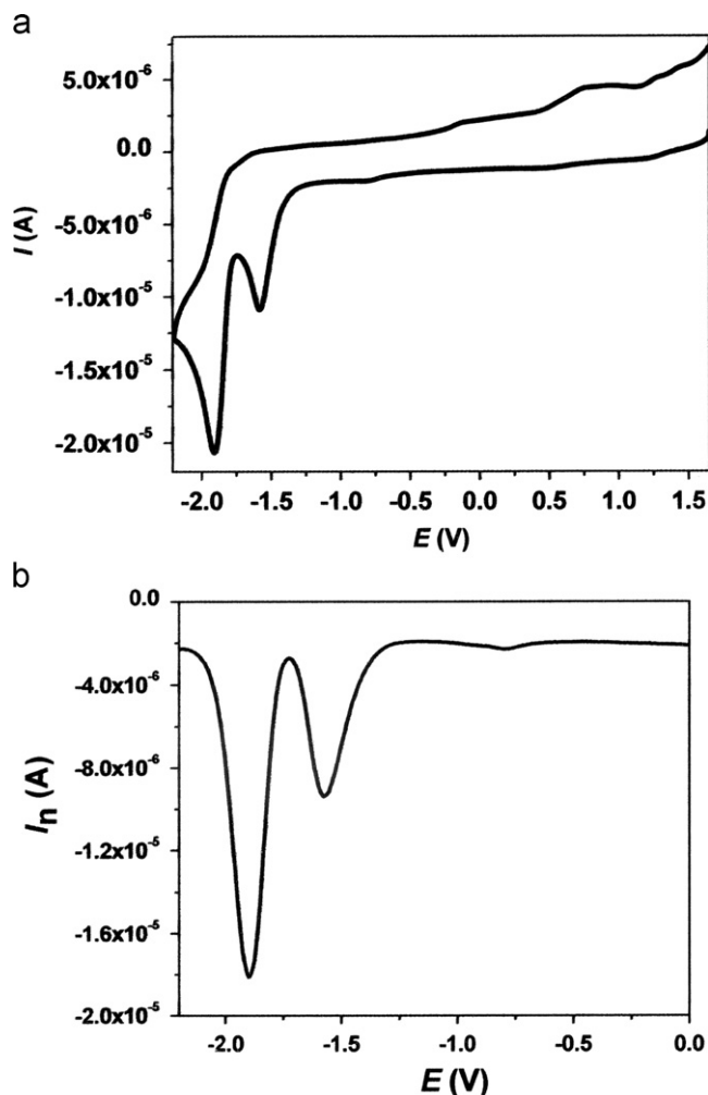
Fig. 6. a) Cyclic and b) SW voltammograms of a mixture of PAT+HMF in ACN+0.1 mol L -1 TBAP at a GC electrode. c_{PAT}^* = 4.0 \times 10^{-4} mol L -1 , c_{HMF}^* = 9.8 \times 10^{-4} mol L -1 , v = 0.050 V s -1 .
