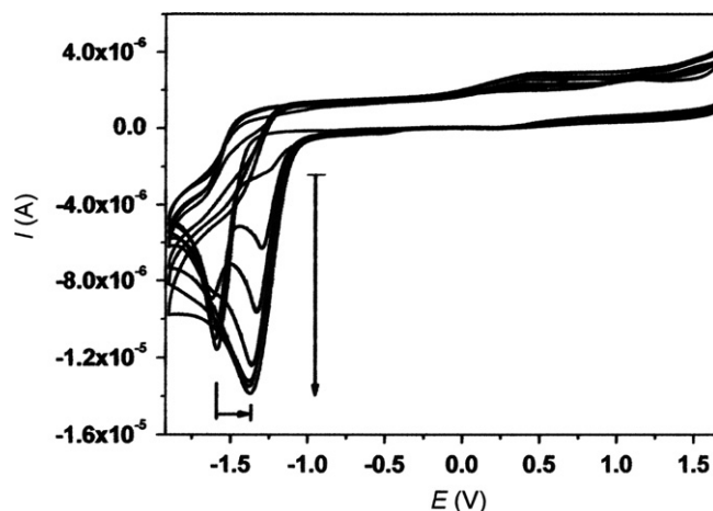
Fig. 4. Cyclic voltammograms of PAT in ACN + 0.1\text{ mol L}^{-1} TBAP in the absence and in the presence of different aliquots of TFA. c_{\text{PAT}}^* = 4.0 \times 10^{-4}\text{ mol L}^{-1} . c_{\text{TFA}}^* was varied from 0 to 1.23 \times 10^{-3}\text{ mol L}^{-1} . v = 0.050\text{ V s}^{-1} . Vertical and horizontal arrows indicate the increase in the current, and the shift of the PAT electro-reduction peak at less cathodic potentials, respectively, as the TFA concentration increases.
